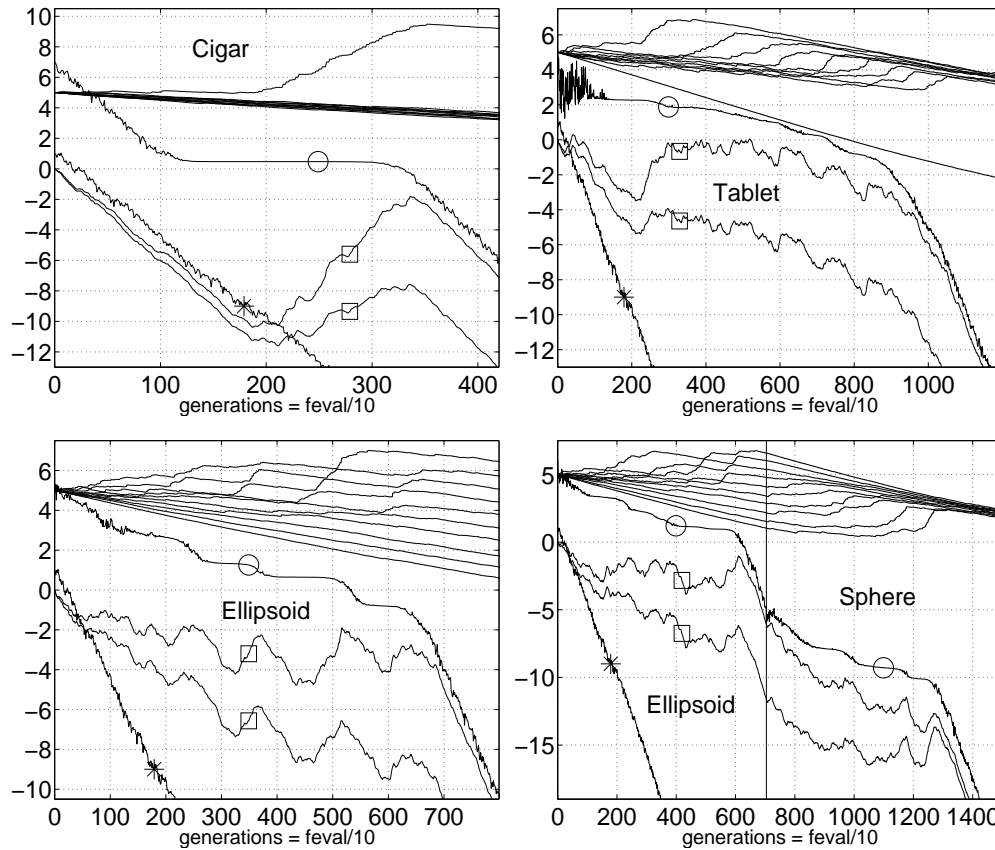
Figure 9: Simulation runs with the (2_1, 10) -CMA-ES, where n = 10 . \circ : \log_{10} (function value). \square : \log_{10} (smallest and largest variance of the mutation distribution), * : \log_{10} (function value) from a run on f_{\text{sphere}} . The upper ten graphs (without symbol) are the variances of the principal axes of the mutation distribution ellipsoid, sorted, and multiplied with 10^5/\sigma(g)^2 on a logarithmic scale. Lower right: Simulation run on f_{\text{elli}} until function value 10^{-5} is reached and afterwards on \text{const} \cdot f_{\text{sphere}} . The CMA-ES meets the adaptation demand. After an adaptation phase, in all cases, the progress rates are identical with those on f_{\text{sphere}} .
