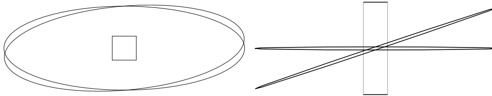
Figure 2: Lines of equal probability density of two normal distributions ( n = 2 ) with axis ratios of 1 : 3 (left) and 1 : 300 (right) before and after rotation by \frac{5}{180}\pi . The right figure is enlarged in the y -direction; the rectangle covers the identical area in the left and in the right. Comparing the cross section areas of the ellipsoids, the distributions with axis ratio of 1 : 3 are very similar, while the distributions with axis ratio 1 : 300 differ substantially.
