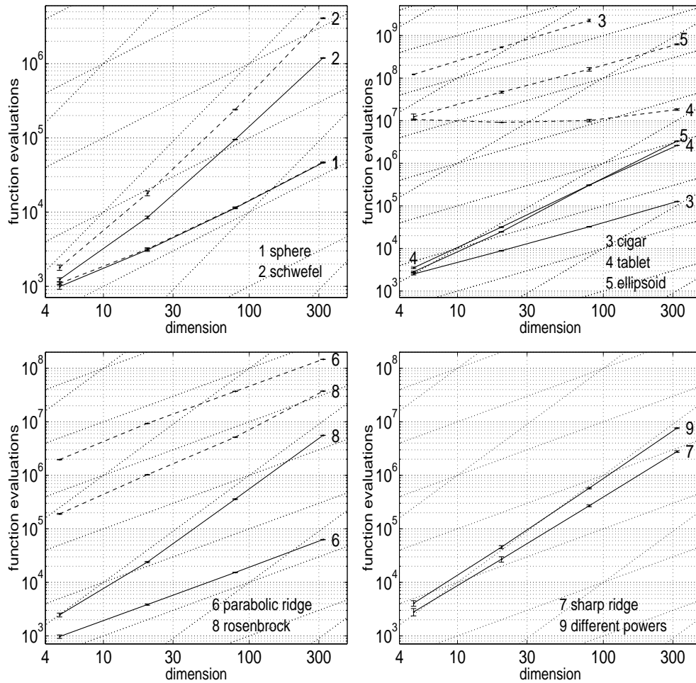
Figure 10: Function evaluations to reach f^{\text{stop}} with the (2_1, 10) -CMA-ES (solid graphs) and the (2_1, 10) -PATH-ES (dashed graphs) vs. dimension n on the test functions 1–9, where n = 5; 20; 80; 320 . Shown are mean values and standard deviations. Sloping dotted lines indicate \text{const} \cdot n = [10; 100; 1000; \dots] \cdot n and \text{const} \cdot n^2 = [1/100; 1; 100; \dots] \cdot n^2 function evaluations. For the PATH-ES the missing result on f_{\text{cigar}} ( n = 320 ) could not be obtained in reasonable time (upper right) and results on f_{\text{sharpR}} and f_{\text{diffpow}} are far above the shown area (lower right, compare text). On f_{\text{sphere}} (upper left), both strategies perform almost identically.
