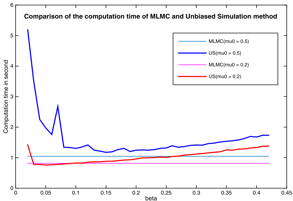
FIG. 1. Comparison of the computation time of MLMC method and unbiased simulation method for problem (4.3), with the same given error.
