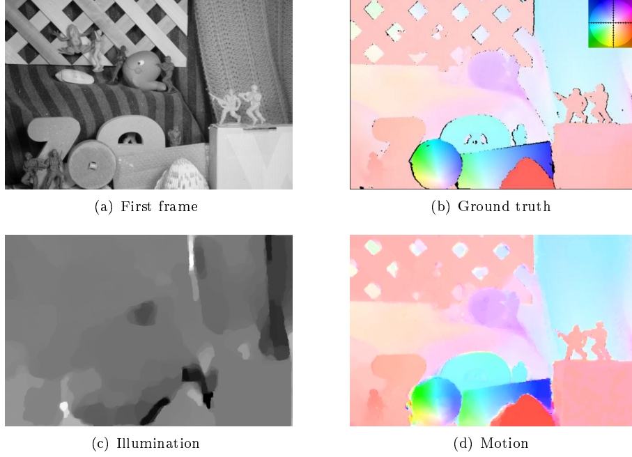
Figure 11: Motion estimation using total variation regularization and explicit illumination estimation. (a) shows one of two 584 \times 388 input images and (b) shows the color coded ground truth motion field (black pixels indicate unknown motion vectors). (c) and (d) shows the estimated illumination and the color coded motion field.
