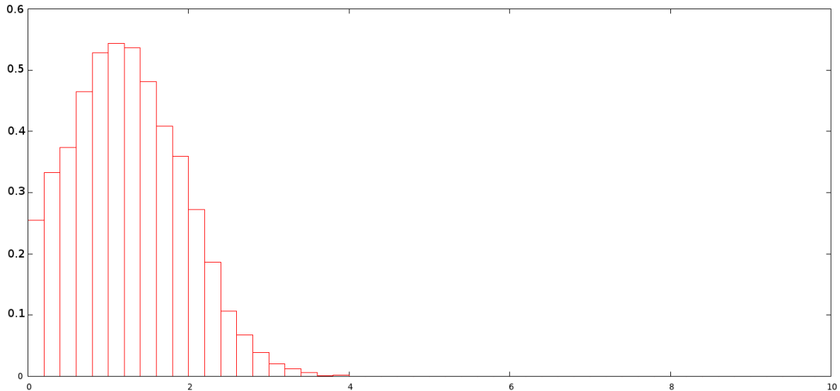
Figure 11: First marginal of the Yaglom limit of a 3-type stochastic Lotka-Volterra system. The two other marginals are equal to the null measure.
