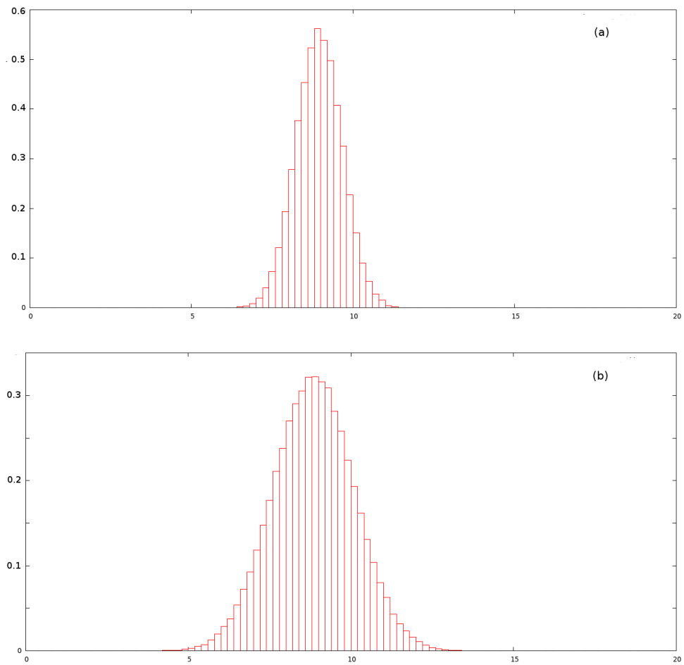
Figure 8: Example 4. The Yaglom limits of two logistic Feller diffusion processes with the same charge capacity: (a) r = 9 and c = 1 ; (b) r = 3 and c = 1/3 .
