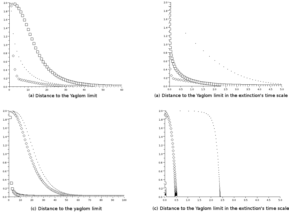
Figure 3: Example 2. Pictures (a) and (c) correspond to different values of \lambda (the following values of \theta(\alpha) - \chi have been obtained by numerical computation): (a) \lambda = 0.9 , \theta(\alpha) = 0.100 , \theta(\alpha) - \chi = 0.102 ; (c) \lambda = 1.1 , \theta(\alpha) = 5.84 \times 10^{-5} , \theta(\alpha) - \chi = 0.103 ; each curve corresponds to a given initial size of the population: (\cdot) Z_0 = 1 ; (\diamond) Z_0 = 10 ; (\square) Z_0 = 100 .
