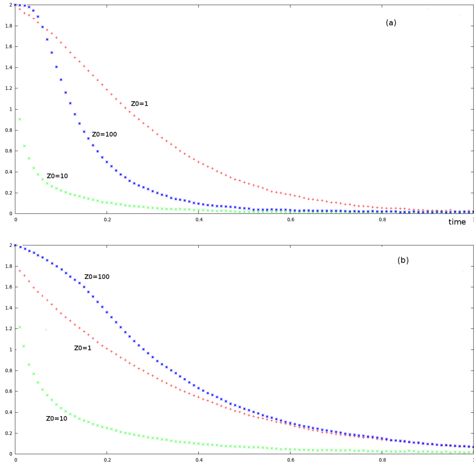
Figure 6: Example 3. Evolution of the distance between the conditioned distribution and the Yaglom limits of two logistic birth and death processes with the same charge capacity \frac{\lambda-\mu}{c} = 9 : (a) \lambda = 10, \mu = 1 and c = 1 ; (b) \lambda = 10, \mu = 7 and c = 1/3 .
