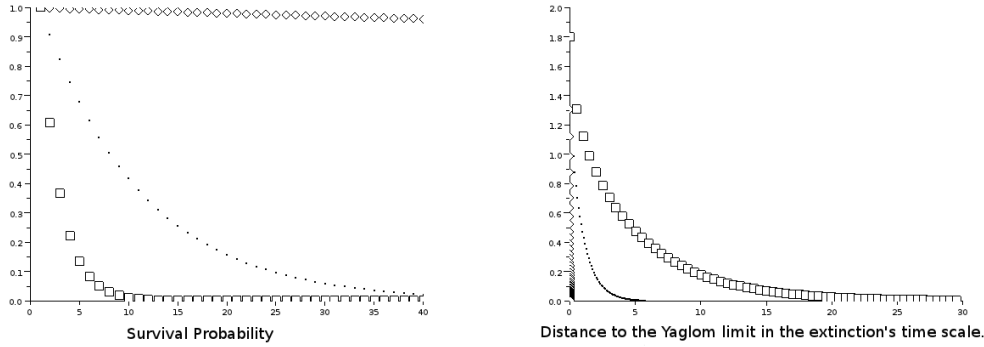
Figure 1: Example 1. A numerical computation leads to \lambda = 0.098 . Three different situations are observed, which lead to three very different patterns for the speed of convergence to the Yaglom limit in the extinction's time scale: ( \diamond ) \lambda \gg d = 0.001 ; ( \square ) \lambda \ll d = 0.500 ; ( \cdot ) \lambda = d = 0.098 .
