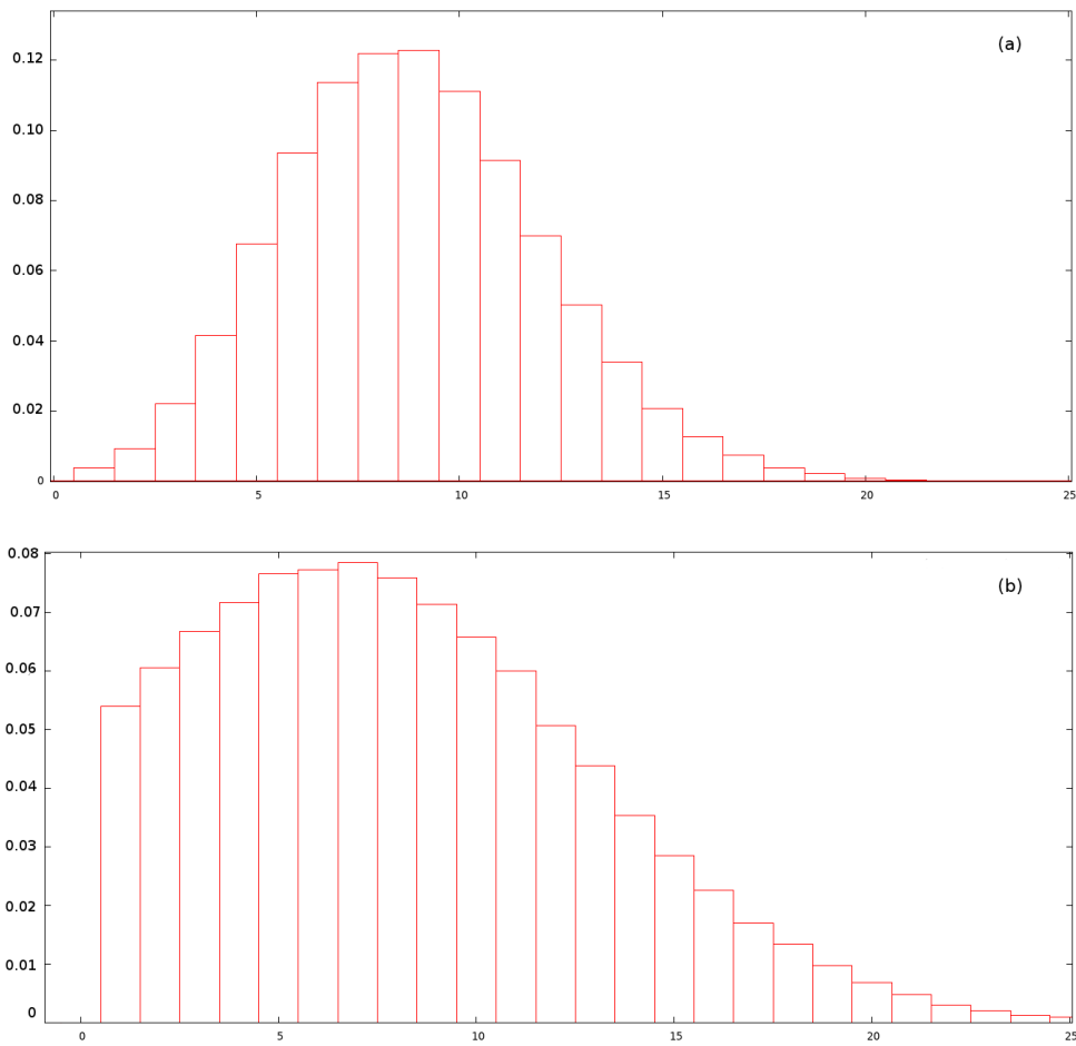
Figure 5: Example 3. The Yaglom limits of two logistic birth and death processes with the same charge capacity \frac{\lambda-\mu}{c} = 9 : (a) \lambda = 10 , \mu = 1 and c = 1 ; (b) \lambda = 10 , \mu = 7 and c = 1/3 .
