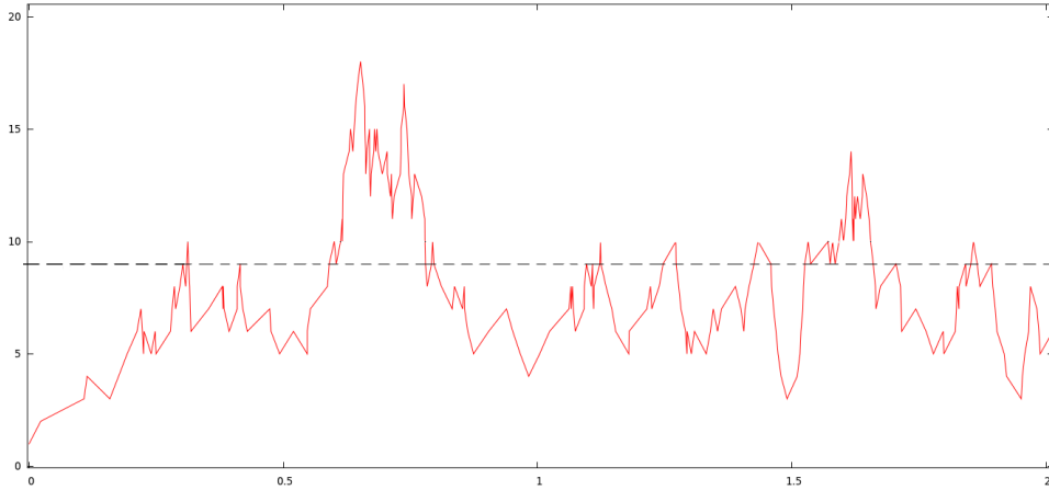
Figure 4: Example 3. A random path of a logistic birth and death process with initial size Z_0 = 1 and with parameters \lambda = 10 , \mu = 1 and c = 1
