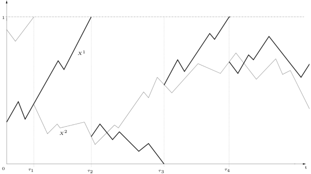
Figure 12: Fleming-Viot type system with two particles absorbed in 0 and 1.
