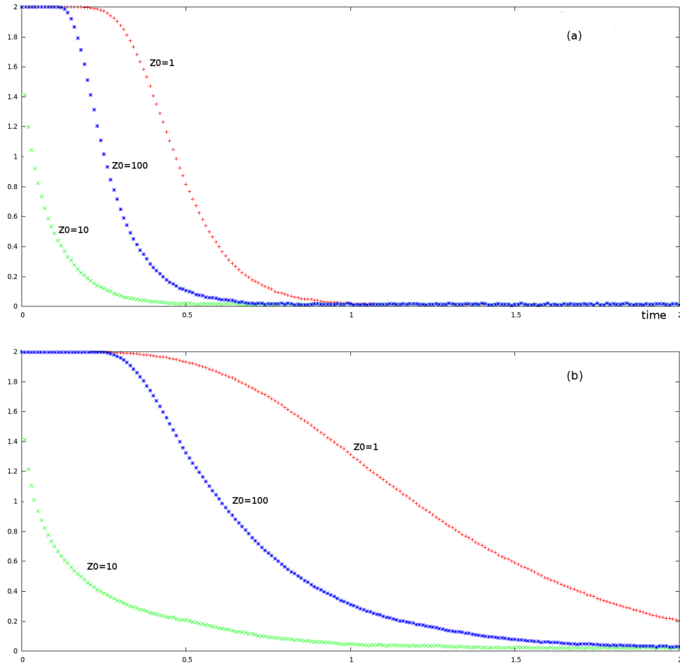
Figure 9: Example 4. Evolution of the distance between the conditioned distribution and the Yaglom limits of two logistic Feller diffusion processes with the same charge capacity \frac{r}{c} = 9 : (a) r = 9 and c = 1 ; (b) r = 3 and c = 1/3 .
