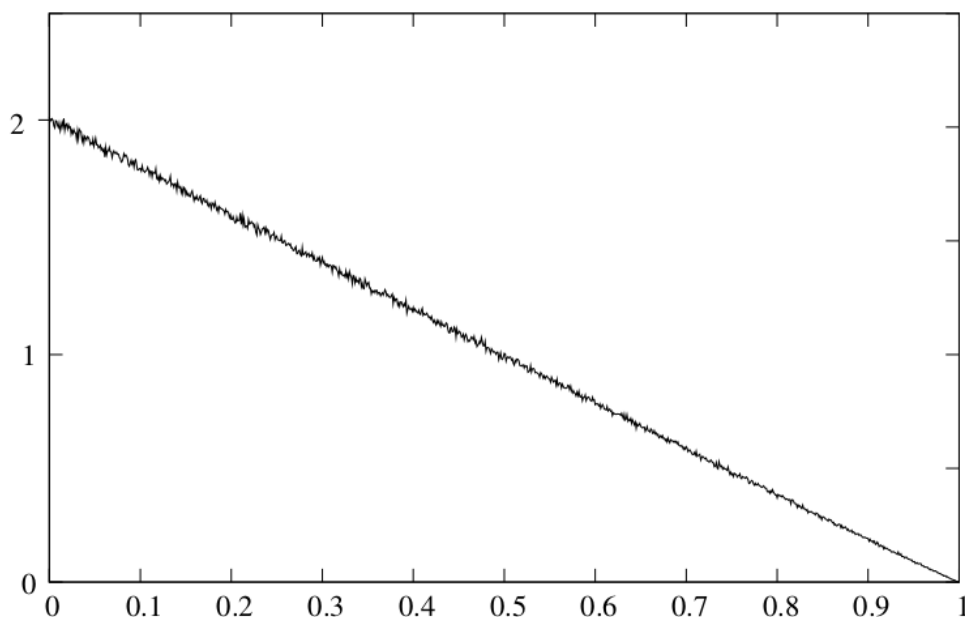
Figure 13: The Yaglom limit of the Wright-Fisher diffusion conditioned to be absorbed at 0 obtained by numerical simulation.
