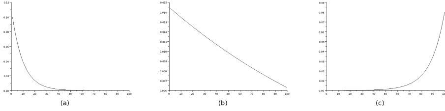
Figure 2: Example 2. Yaglom limits for different values of \lambda . The following values of \theta(\alpha) are obtained by numerical computation. (a) \lambda = 0.9 , \theta(\alpha) = 0.100 ; (b) \lambda = 1.0 , \theta(\alpha) = 0.014 ; (c) \lambda = 1.1 , \theta(\alpha) = 5.84 \times 10^{-5} .
