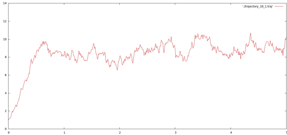
Figure 7: Example 4. A random path for logistic Feller diffusion process with initial size Z_0 = 1 and parameters r = 9 and c = 1
