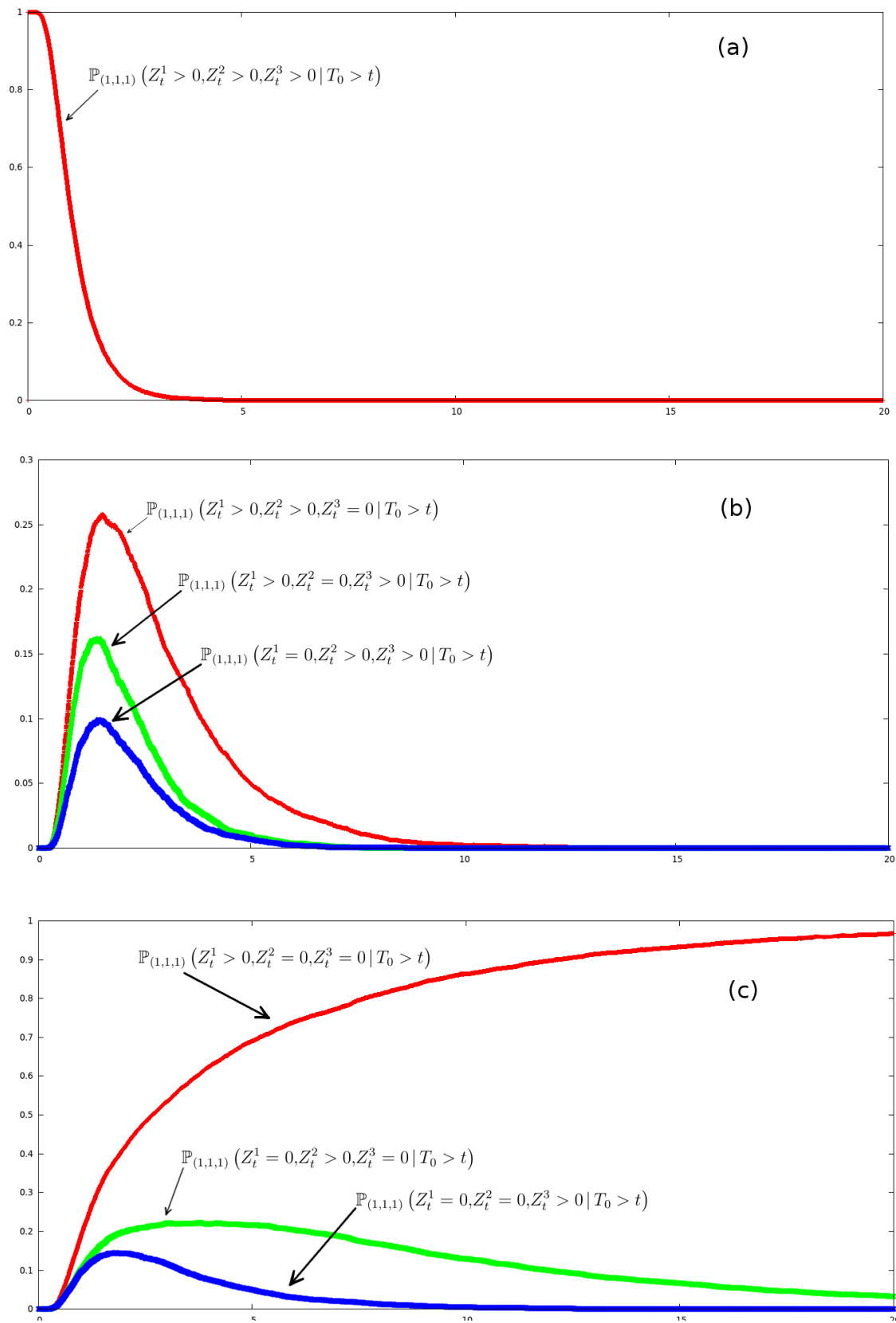
Figure 10: Dynamics of the probabilities of co-existence and existence of the different types for a 3-type stochastic Lotka-Volterra system. The horizontal axis is the time axis
