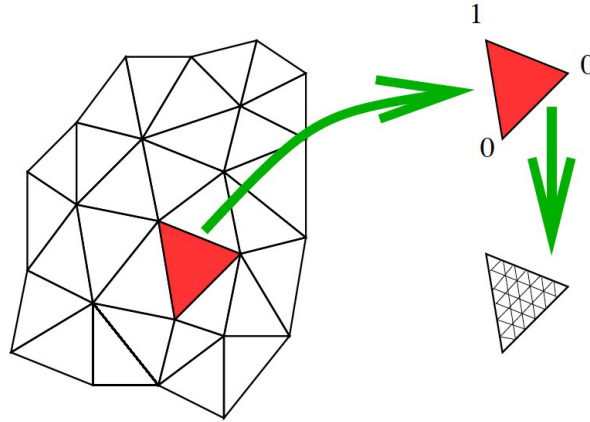
Figure 6.1: The multiscale Finite Element Method. On the mesh, one computes the base functions as oscillating solutions on a thinner mesh.
