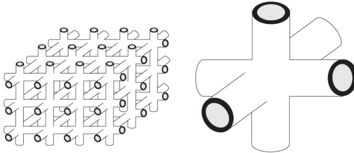
Figure 5.3: In 3d, it is possible to have a fluid and a solid domains that are both connected. An example is given by the periodic structure shown on the left and made by repetitions of the unit structure to the right (from [15]).
