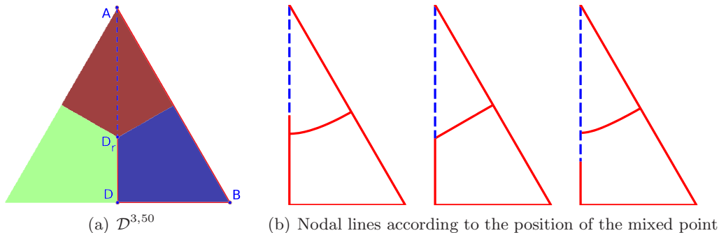
FIGURE 6. Dirichlet-Neumann approach for 3-partitions of the equilateral triangle.
