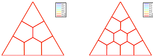
FIGURE 21. p -minimal k -partitions of the equilateral triangle vs. p , for k \in \{6, 10\} .
