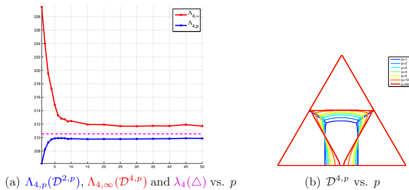
FIGURE 19. p -minimal 4-partitions of the equilateral triangle vs. p .
