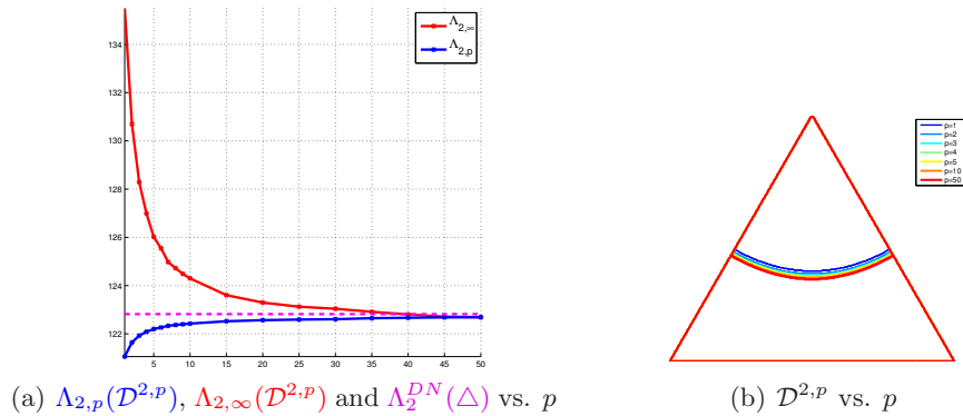
FIGURE 18. p -minimal 2-partitions of the equilateral triangle vs. p .
