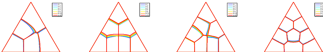
FIGURE 20. p -minimal k -partitions of the equilateral triangle vs. p , for k \in \{5, 7, 8, 9\} .
