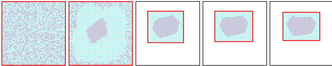
FIGURE 1. Evolution of the local grid for a cell for iterations 1, 10, 25, 45, 85. This computation corresponds to k = 10 and p = 1 .
