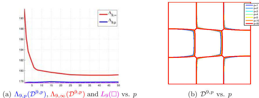
FIGURE 25. p -minimal 9-partitions of the square vs. p .
