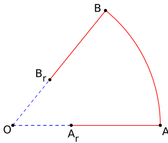
FIGURE 9. The setup for the mixed problem on sectors.
