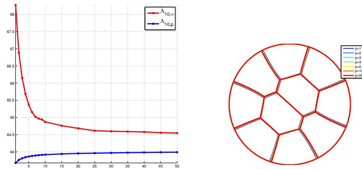
FIGURE 28. p -minimal 10-partitions of the disk vs. p .
