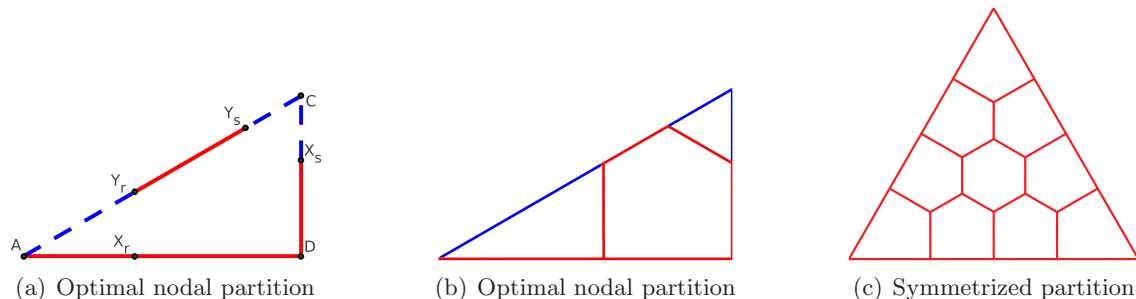
FIGURE 15. Dirichlet-Neumann approach for 10-partitions of the equilateral triangle.
