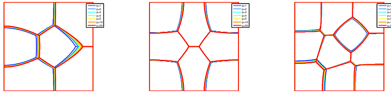
FIGURE 24. p -minimal k -partitions of the square vs. p , for k \in \{6, 8, 10\} .
