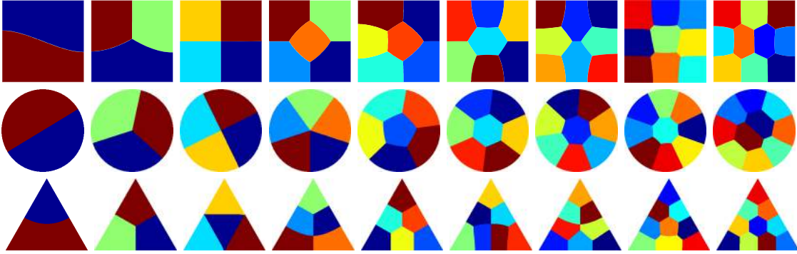
FIGURE 5. Partitions obtained with the penalization method.
