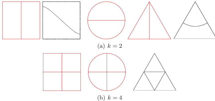
FIGURE 4. Nodal \infty -minimal k -partitions, k = 2, 4
