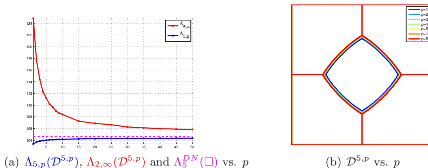
FIGURE 23. p -minimal 5-partitions of the square vs. p .
