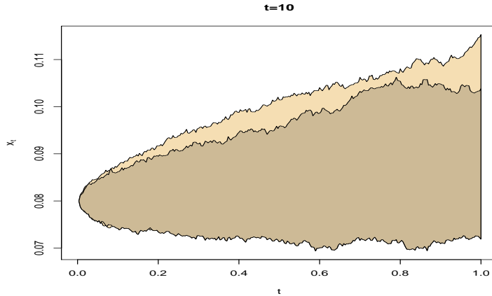
Figure 2: Cox-Ingersoll-Ross European option simulation: range of N simulated process (r_{pT/n}^n)_{1 \leq p \leq n} ( lighter background ) compared with the corresponding N resampled process (\tilde{r}_{pT/n}^n)_{1 \leq p \leq n} ( darker background ) for K = 0.09 , using a D = 3 -kernel PMC algorithm with \theta = 0 , \theta = 1 and \theta = 2 , T = 10 iterations and N = 10,000 simulations.
