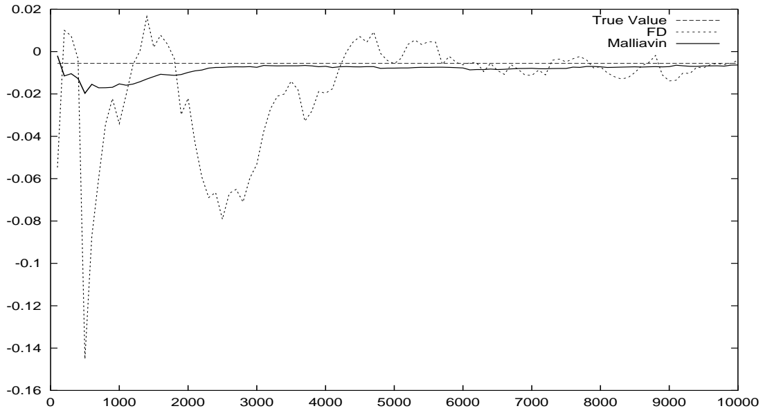
Figure 2: Gamma of an up & out Call.
