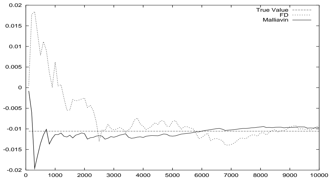
Figure 3: Delta of an up & out Call, using the extrema process.
