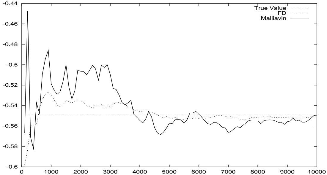
Figure 4: Delta of an lookback Put.
