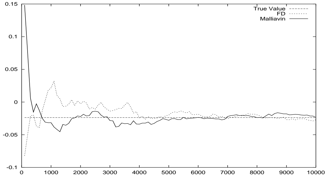
Figure 1: Delta of an up & out Call, using the averaged modulus continuity process.
