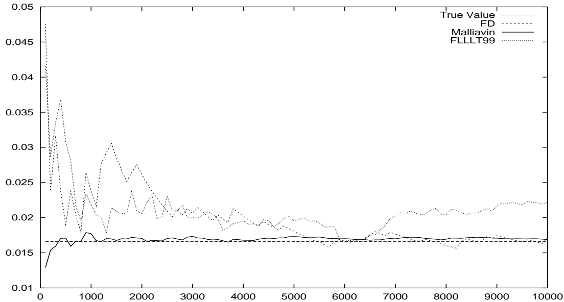
Figure 5: Delta of up in & down out digital Call.
