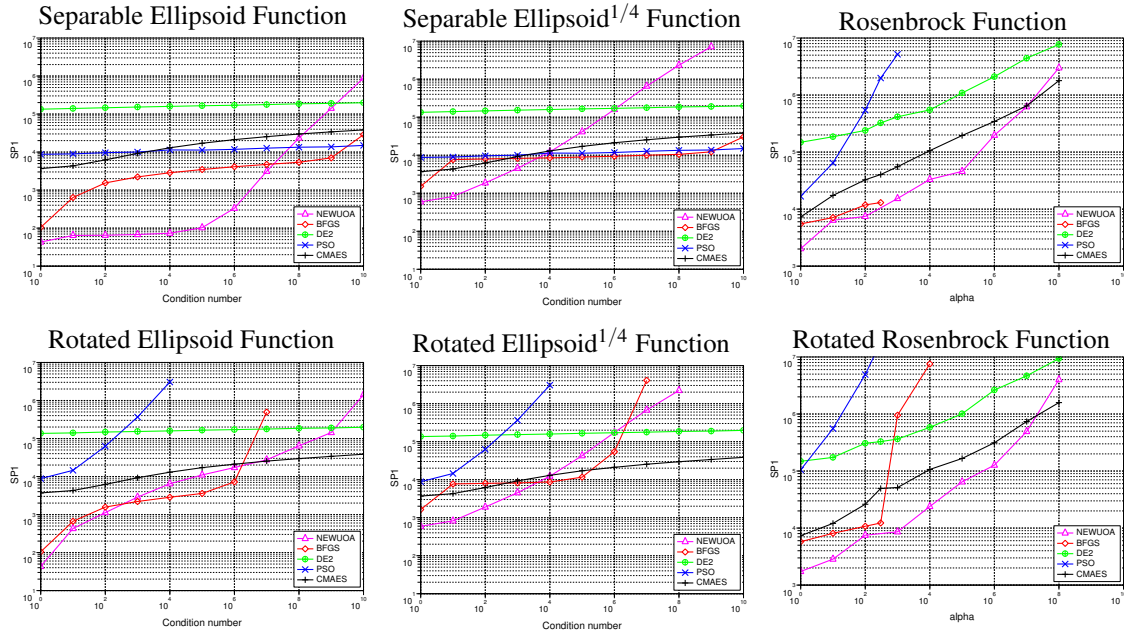
Figure 1: Ellipsoidal functions in 20D (1st and 2nd columns). Shown is SP1 (the expected running time or number of function evaluations to reach the target function value) versus condition number. Rosenbrock function (3rd column). Shown is SP1 versus conditioning parameter \alpha .
