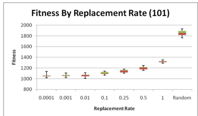
Figure 12. Fitness by replacement rate over 500,000 generations for 101 city TSP at a mutation rate of 0.8%.
