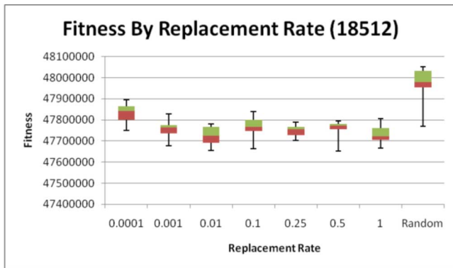
Figure 14. Fitness by replacement rate over 2,000,000 generations for 18,512 city TSP at a mutation rate of 0.01%.
