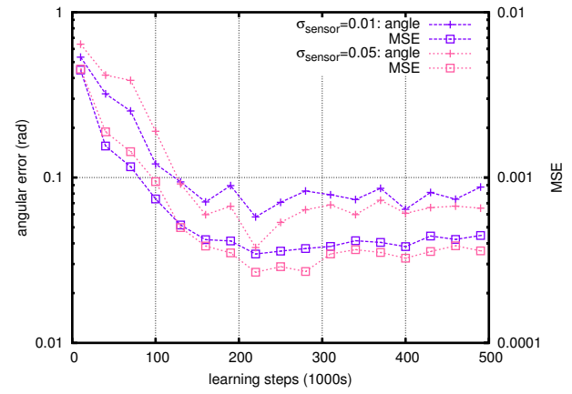
(b) Kalman Filtering
