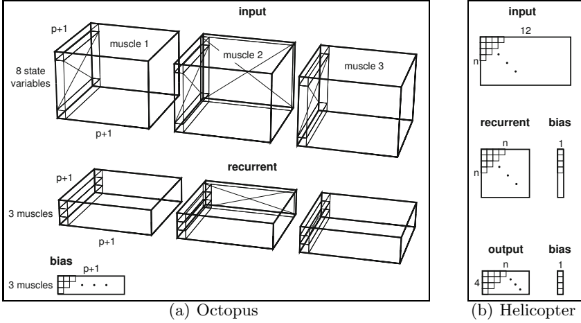
Fig. 4. Network decoding schemes. (a) for the octopus arm networks the genome is split into 3 chromosomes, \Omega=\{4, 4, 2\} . The coefficients in the chromosome used to generate the input weight matrix are placed in a 4D array, and a 2D array for the bias weights. (b) for the helicopter networks there are 5 chromosomes, \Omega=\{2, 2, 1, 2, 1\} : a 2D input and recurrent and output arrays, and 1D arrays for the input and output bias weights.
