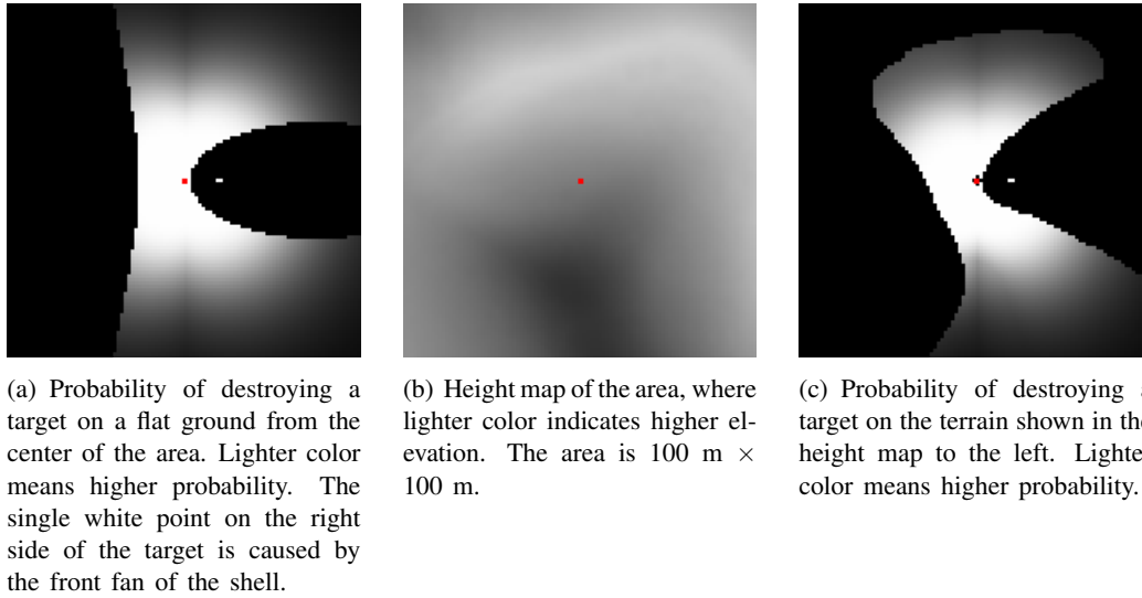
Figure 4: The terrain changes the probability of destroying a target when the shell explodes in the center of the area, indicated by a red dot. The point of burst is located in the center of the figure, indicated by a red dot. The round is fired from the east with 45^\circ angle of fall and explodes 10 m above the ground. The kill probability is For some areas the kill probability drops to 0 because of the geometry of the fragment fans and the cover provided by the terrain, and the difference in explosion height changes the effective ranges of the fragment fans. Figure 4(a) shows the probability of destroying a target on flat terrain, and Figure 4(c) shows the probabilities when considering the terrain shown in Figure 4(b).
