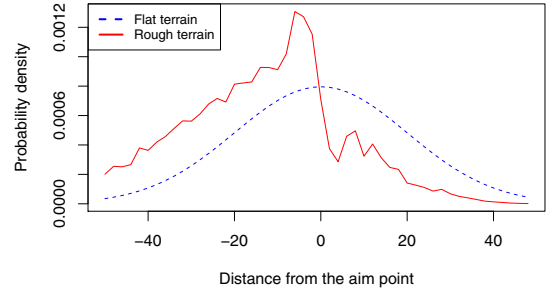
(b) Impact distribution of rounds on flat terrain and on the rough terrain in Figure 3(a).
