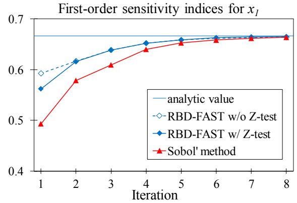
Figure 6: First-order sensitivities for x_1 calculated with RBD-FAST and the Sobol' method, respect.
