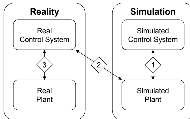
Figure 3: Emulation (Smith and Cho 2008)
