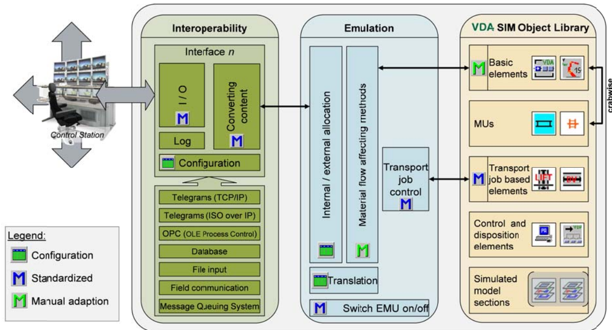
Figure 5: Adding emulation functionality to the VDA automotive object library
