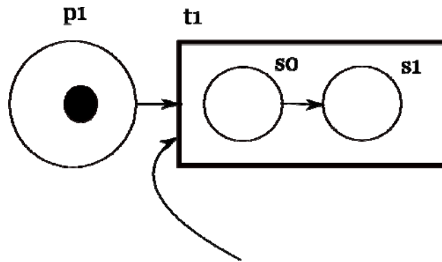
Figure 4: A part of the Petri net in Figure 3 where transition t1 is refined as a state machine
