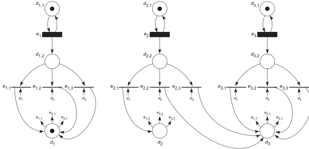
Figure 3: Alternative representation of SPN with a transient marking.
