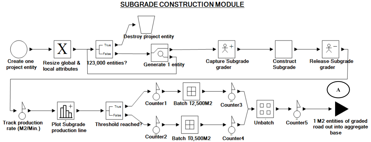
Figure 6: A model for the subgrade construction process
