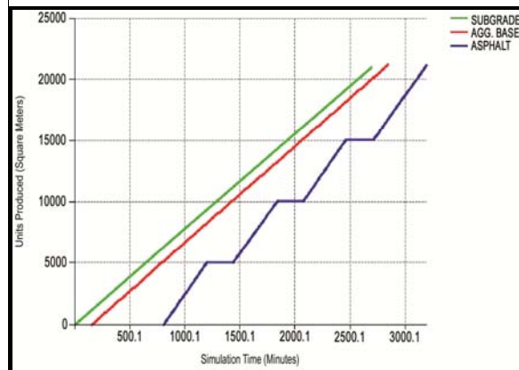
Figure 9b: Line of balance from GPS
