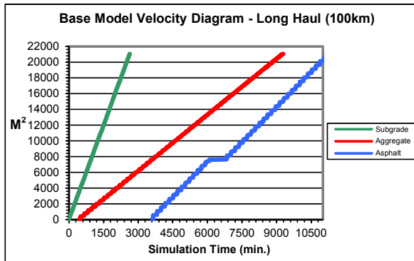
Figure 10a: Line of balance from SWRC template
