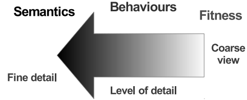
Figure 1: Conceptual view of how the performance of a program can be analyzed. At one extreme we have fitness-based analysis, a coarse view of performance. Semantics lies at another extreme, where a high level of detail is sought. Finally, behavioral analysis provides a variable scale based on how context is considered.
