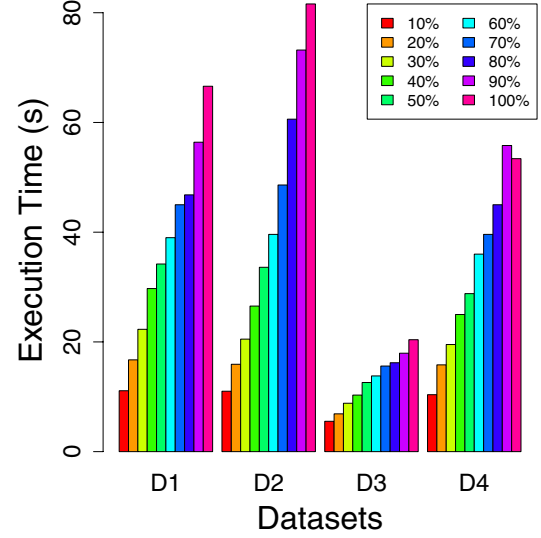
Figure 2: Execution time
