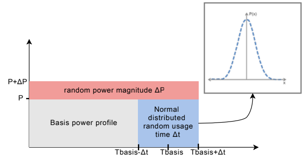
Figure 2: Each appliance power profile is defined by its power magnitude P and its base usage time t_{basis} . Due to the fact that usage times are not constant in reality, we vary the usage time by a normal distributed time variable \Delta t , which is added/subtracted to/from the basis/ mean base usage time, t_{basis} or a gamma distributed time ( \Gamma(\alpha = 2, \beta = 50) ) variable, which is added to the base usage time t_{basis} . Beside the usage, also the power is diversified as we vary the power P with an additional uniform distributed random variable, \Delta P .
