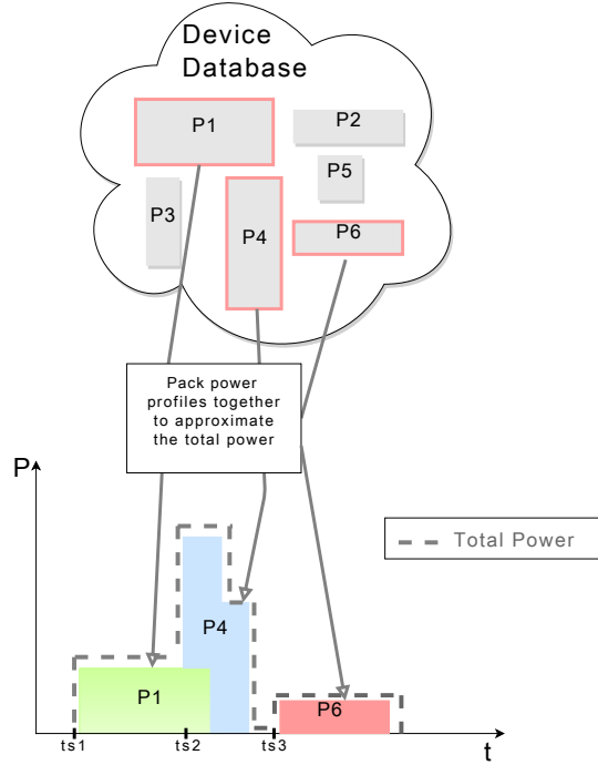
Figure 1: Basic principle of the ON/OFF time genome appliance detection. Find a composition of saved power profiles P_i , place it at the switching times t_s and try to minimize the error between the evolved power load and the given total power load.
