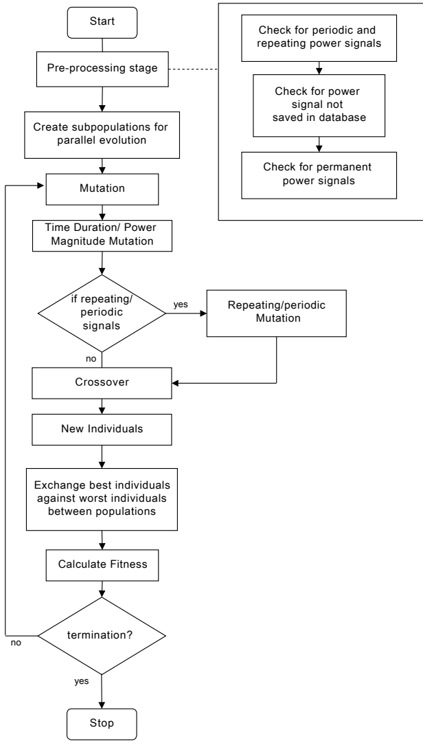
Figure 3: General scheme of the evoNILM algorithm as a flowchart
