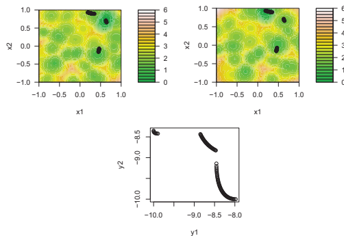
Figure : Pareto front and set with 30 degree rotation.
