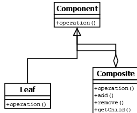
Figure 1: UML class diagram of composite pattern
