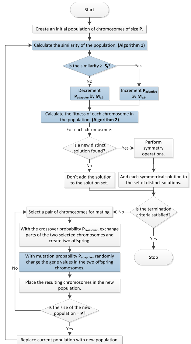
Fig. 3. Self-Adaptive GA Flowchart
