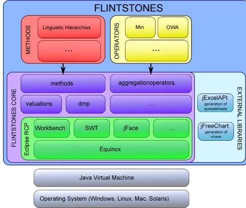
Fig. 1. Flintstones architecture
