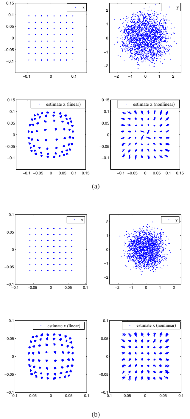
Fig. 3. Effectiveness of the proposed nonlinear SC-FDE scheme based on the estimated CIR \hat{\mathbf{h}} and the estimated HPA's CV static nonlinearity as well as the estimated inverse mapping for the HPA's amplitude response under: (a) \text{OBO} = 3 \text{ dB} and E_b/N_o = 10 \text{ dB} ; and (b) \text{OBO} = 5 \text{ dB} and E_b/N_o = 4 \text{ dB} . The top two plots in sub-figures (a) and (b) depict one transmitted QAM symbol block \mathbf{x} and its received signal block \mathbf{y} , while the bottom two plots show the corresponding estimated \hat{\mathbf{x}} obtained by the linear and nonlinear SC-FDEs, respectively.
