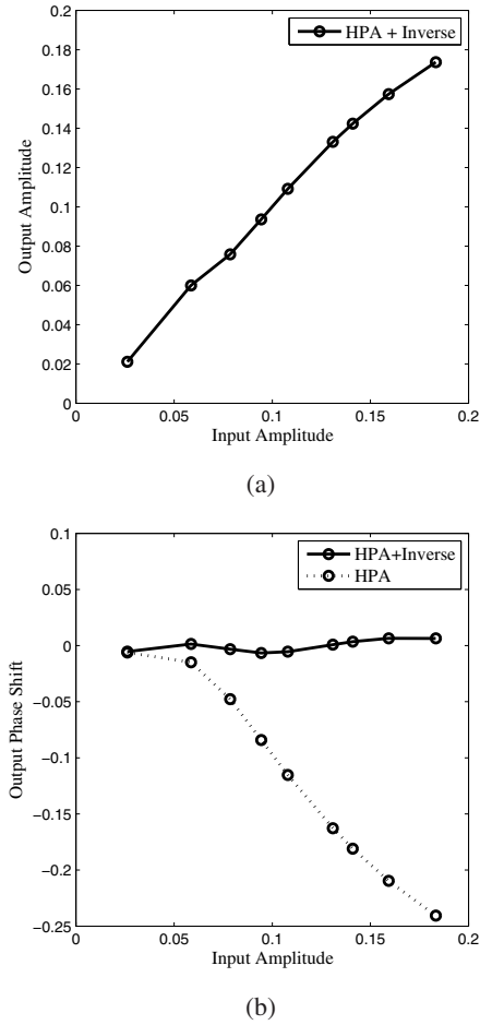
Fig. 2. Combined response of the true HPA and its estimated inversion obtained under \text{OBO} = 2 \text{ dB} and E_b/N_o = 10 \text{ dB} : (a) combined amplitude response, and (b) combined phase response.
