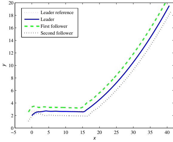
Fig. 2. Formation trajectories
