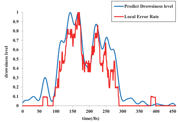
Fig. 8. An example of the regression result of a subject. The predicted drowsiness curve in blue seizes the tendency of local error rate and perfectly reflects the states of the subject.
