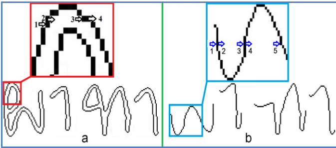
Fig. 5a. Example of transitions on full boundary image and Fig. 5b. example of transitions on lower contour .
