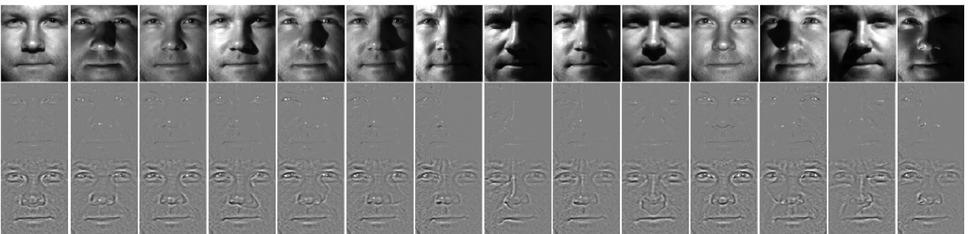
Fig. 4. The comparison of two methods. Top row: the raw images of a single subject from Yale Database B with various illumination conditions; Middle row: the small scale from the TV method with \lambda = 0.6 ; Bottom row: the high frequency using the TV-NSCT method with \lambda = 0.6 .
