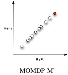
Fig. 1. An example of the quality of policies given their return in MDP M , and its multi-objectivized version M' . The total order over policies is preserved.
