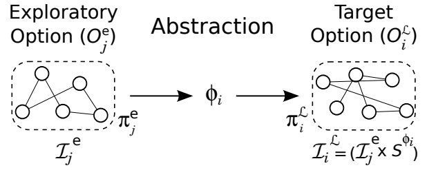
Fig. 4. Once an abstraction \phi_i is learned corresponding to an exploratory-option stream \mathbf{x}_j = \mathcal{U}(\mathcal{P}(s, \pi_j^e(s^\dagger))) , its feature-activation values are quantized to a set of discrete feature-states \mathcal{S}^{\phi_i} . A target option is then constructed with the product state-space \mathcal{I}_i^L = (\mathcal{I}_j^e \times \mathcal{S}^{\phi_i}) and a learned target-policy \pi_i^L .
