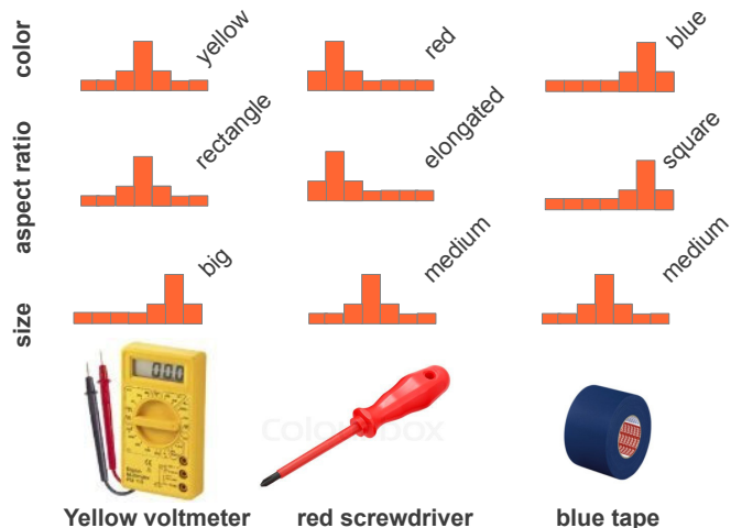
Fig. 2. Simplified synthetic object recognition task: objects and their visual properties (expressed as feature histograms) in the three modalities color, aspect ratio and size. Please note the overlap in the "size" modality between screwdriver and tape, leading to potential ambiguities in feedforward processing.
