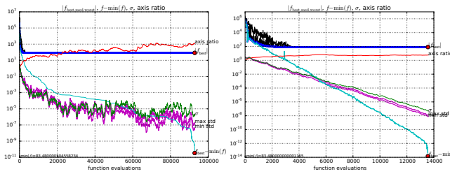
Figure 2: Single runs of IPOP-CMA-MSR (left) and IPOP-CMA-CSA (right) on one instance of the attractive sector function in 20-D. x -axis shows function evaluations. Line with dots (blue): best f -value of the iteration in absolute value, median and worst displayed in thin black lines; cyan line: difference between current f -value and f_{\text{opt}} ; green line: step-size \sigma_t , largest and smallest coordinate-wise standard deviation of the sample distribution in purple; red line: square root of the condition number of the covariance matrix.
