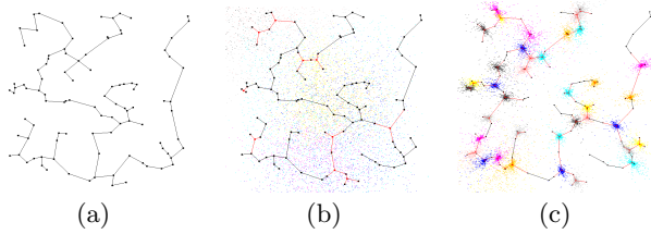
Figure 1: (a) the initial MST without any additional Steiner point; (b) 10 sub-swarms and their best representative as Steiner points: the sub-swarms are still dispersed; (c) the sub-swarms converge: the current solution is close to optimal.
