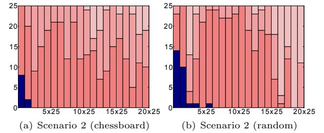
Figure 7: Exemplary development of operator frequencies applied every 25 generations during optimization with the (1+\lambda) -ES on Scenario 2 with (a) chessboard and (b) random initialization.
