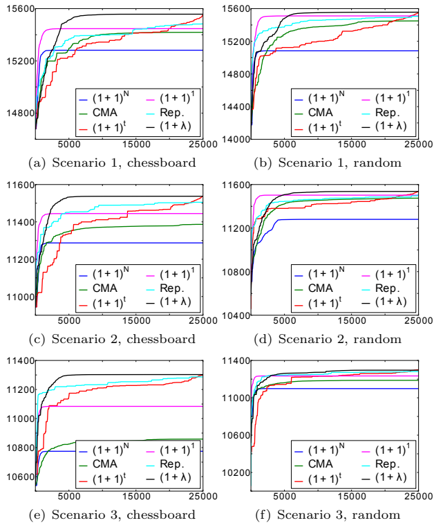
Figure 6: Development of best evolutionary runs when optimizing Scenarios 1, 2, and 3 with chessboard and random initialization. On the y-axis we show the energy output of the wind farm after x fitness evaluations.
