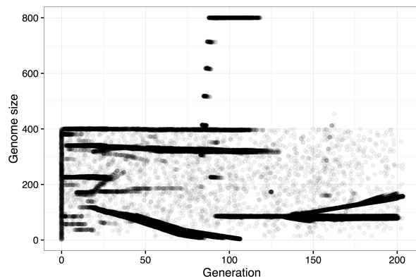
Figure 4: Genome sizes during a single autoconstructive run of GP on the Replace Space With Newline problem
