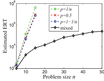
Fig. 1. Estimated ERT of \text{GSEMO}_{mixed} and \text{GSEMO}_p for solving the PL problem, where a base 10 logarithmic scale is used for the y -axis.
