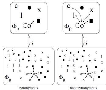
Effects of small mutation steps
