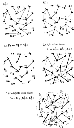
Figure 2: An example for edge crossover ( d = 3 ).
