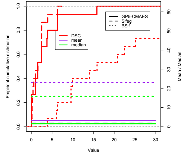
Figure 1: Empirical cumulative distributions (step functions) and means and medians (horizontal lines) for f_{13}
