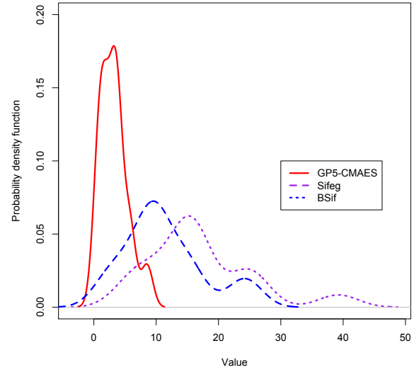
Figure 3: Probability density functions of multiple runs for each algorithm obtained on f_{18}
