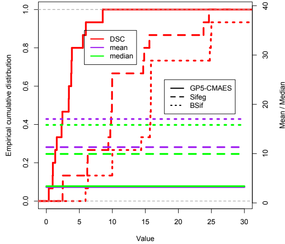
Figure 2: Empirical cumulative distributions (step functions) and means and medians (horizontal lines) for f_{18}
