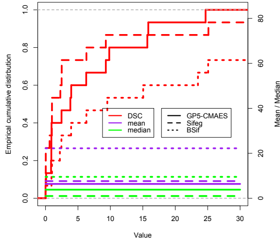
Figure 4: Empirical cumulative distributions (step functions) and means and medians (horizontal lines) for f_{22}
