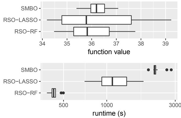
Figure 2: Algorithm comparison on the SCPD-Problem. Upper plots show the performance in terms of best found function value, the lower plots show the total runtime of the algorithms. Lower values are better, thus more to the left is better in the figures.
