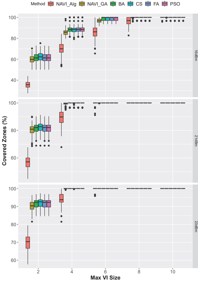
Figure 2: Boxplot for the covered area results. The Y axis represents the covered area, the X axis the MVIS, the panels the MTxP and the series the methods compared.
