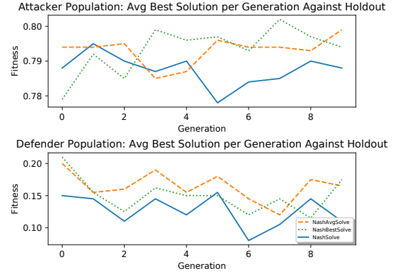
Figure 6: NashSolve variations' performances against the holdout set over time on MAP topology 2 with (population_size=10, generations=10), averaged over 30 runs
