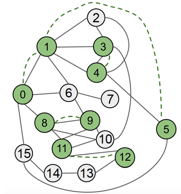
Figure 5: High performing defender on MAP topology 4 with ( p = 20, g = 5 ), green marks the tasks and the dashed line the connections.
