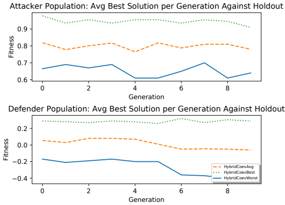
Figure 7: HybridCoev score performance variations against the hold-out set over time on MAP topology 2 with (population_size=10, generations=10), averaged over 30 runs
