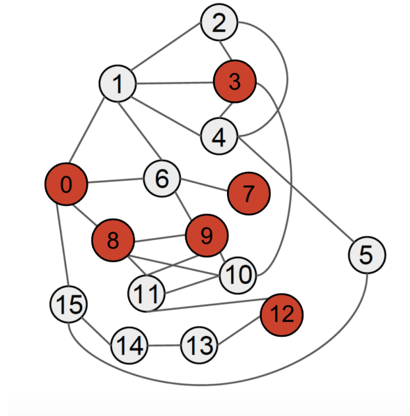
Figure 4: High performing attacker on MAP topology 4 with ( p = 20, g = 5 ), red marks the attacked nodes.
