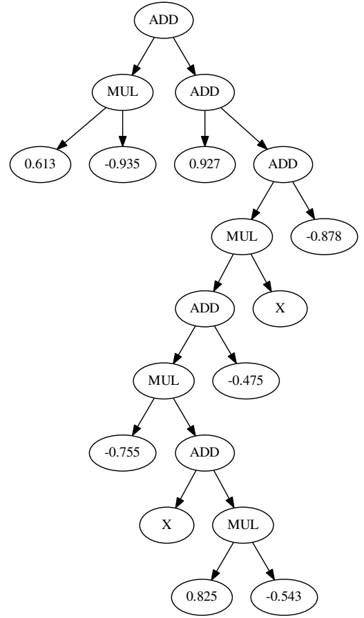
Figure 1: Example subexpression (0.613 \times -0.935) + 0.927 + (-0.755 \times (x + (0.825 \times -0.543))) - 0.475)x - 0.878 as a tree (fun 0 from Table 1). The value of the expression is given by the root node, here ADD, at the top. And plotted as an inverted parabolic red line with + in Figure 3.
