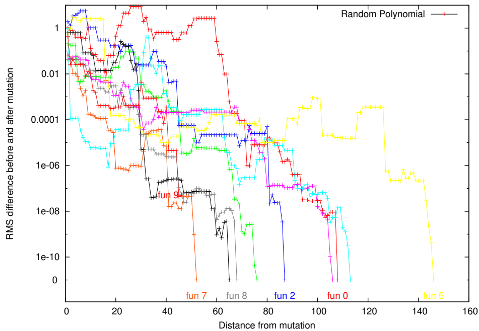
Figure 6: Impact of ten changes against distance from change location. (Impact measured by root mean squared difference on 1001 test cases.) Only fun 9 does not reach zero (RMS difference 5 \cdot 10^{-8} at root node). Colours are the same as in Figure 3, etc. Note non-linear vertical scale.
