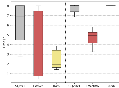
Figure 2: The time needed for each distributed model solving the monolithic use-case to end. All runs were capped at 8 hours maximum.
